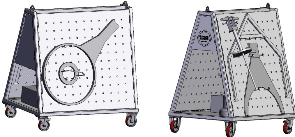
Picture of the tool trolley.
