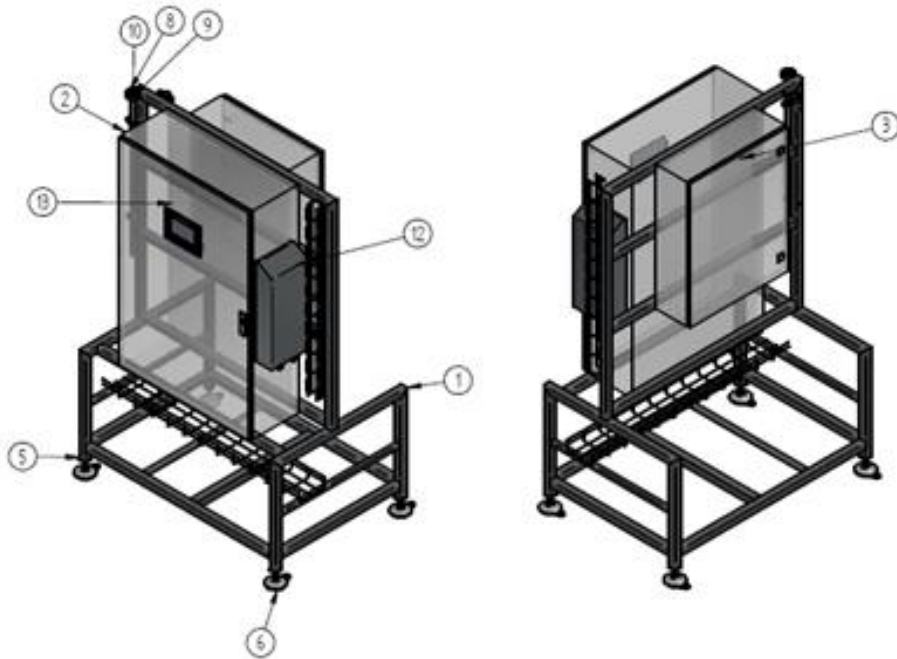
Picture of the control panel
